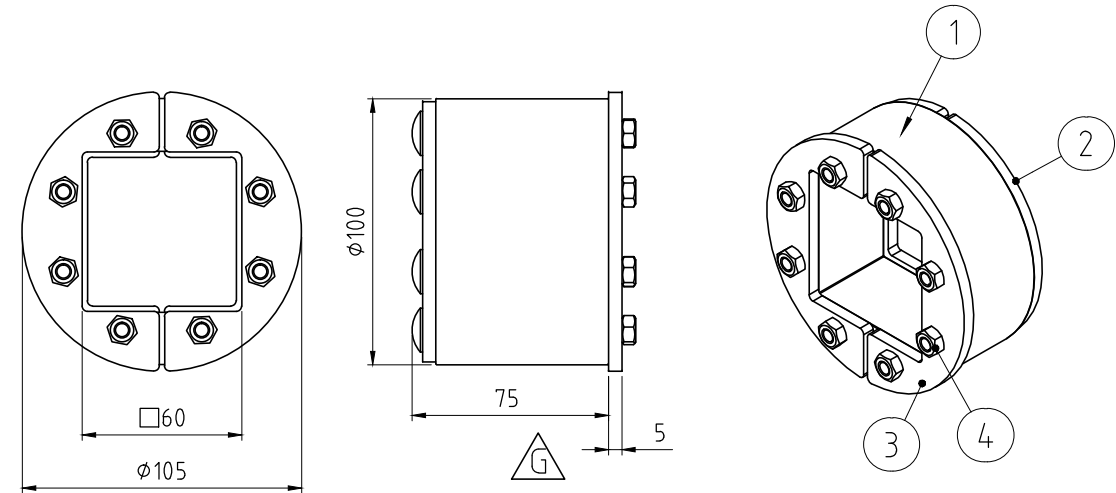
R 100 UG FRAME
